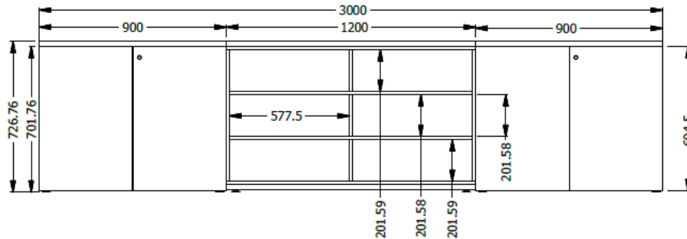
VISTA FRONTAL
